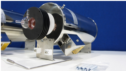
S35-01A Furnace with silica reaction
